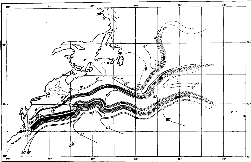
Fig. 1. Schematic chart of temperatures ( ^{\circ}\text{C.} ) at a depth of 200 meters in the Gulf Stream Area.
