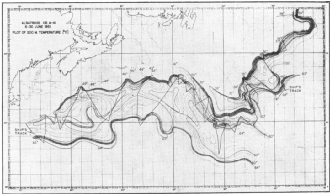
Fig. 2. Temperatures ( ^{\circ}\text{F}. ) at a depth of 200 meters in the Gulf Stream Area. An interpretation of the data obtained on the ALBATROSS III cruise of June 1951.
